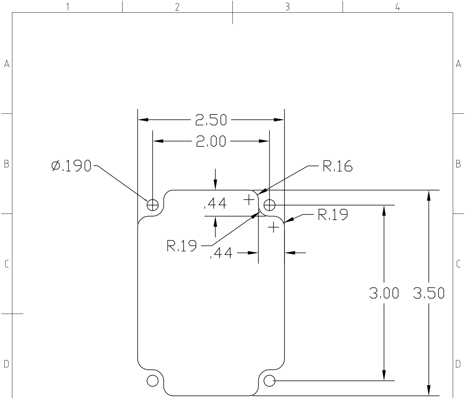
PUMP PANEL CUT OUT DIMENSIONS
