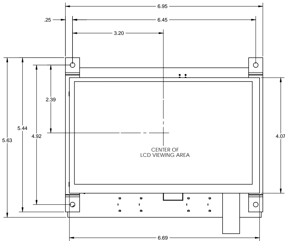
FRONT VIEW
